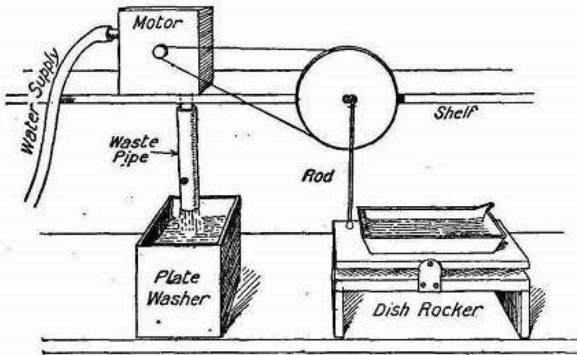
FIG. 108.—Water motor working a photographic dish-rocker.
